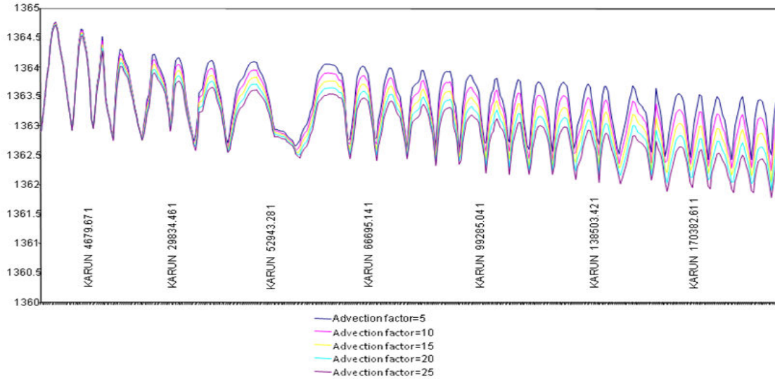
Figure 3: Comparison between different advectios coefficient during a year along the Karoon River
