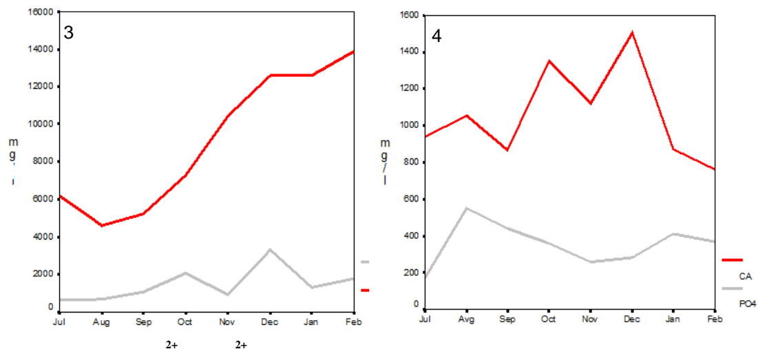
Figure 3: PO 4 and Ca changes in Urmia Lake during the study period
