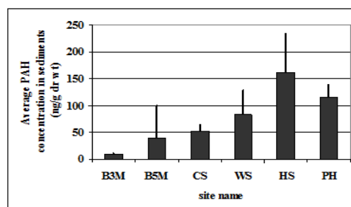
Figure 6: Total average PAH concentration in sediments of sampling sites
