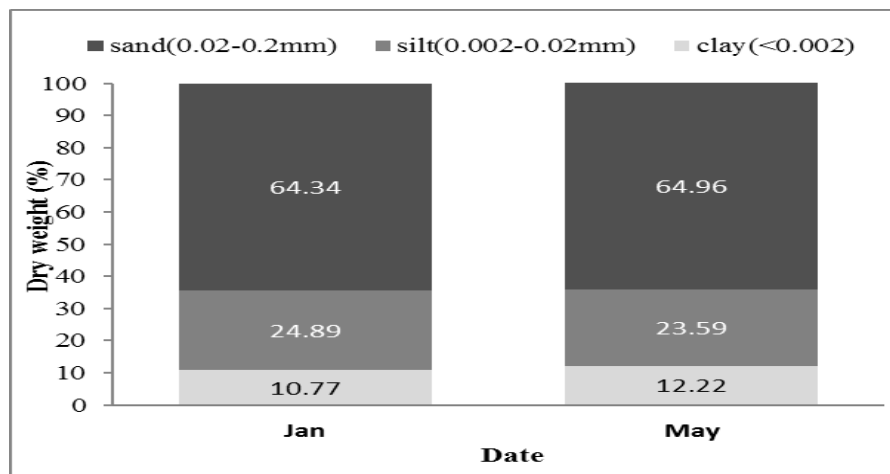
Figure 4: Granulometric structure of sediments expressed as the relative abundance (dry weight percentage) of the different grain-size fractions of samples in the Nashtaroud area.
