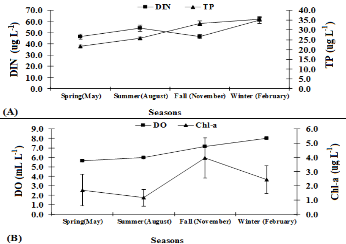
Figure 2: Seasonal changes in the mean concentrations of environmental parameters collected from four transects in ICWCS (2013-2014). (A) DIN and TP; (B) DO and Chl-a.
