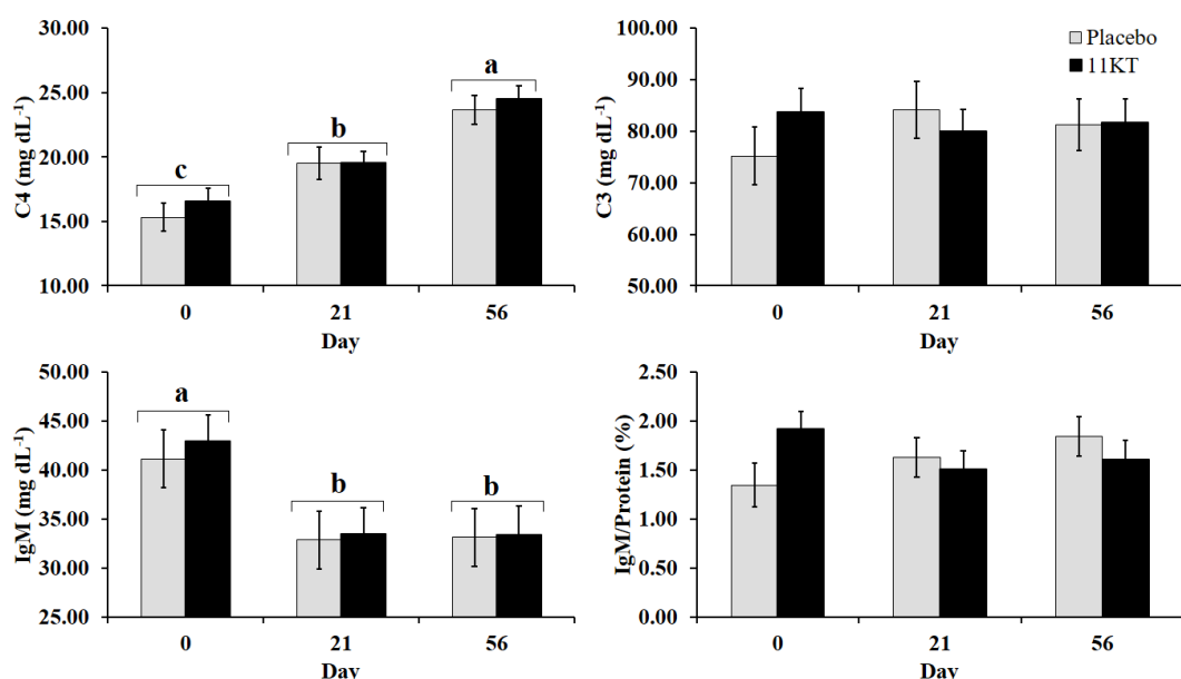
Figure 1: Effects of 11-KT implantation on innate immunity of blood serum in great sturgeon ( Huso huso ) on days 0 (before implantation), 21 and 56 of the experimental period (mean ± SE, n=6). Letters denote statistically significant differences (Two-way ANOVA, p < 0.05 ) with respect to the time effect (no significant difference between the placebo and 11-KT groups in each stage).
