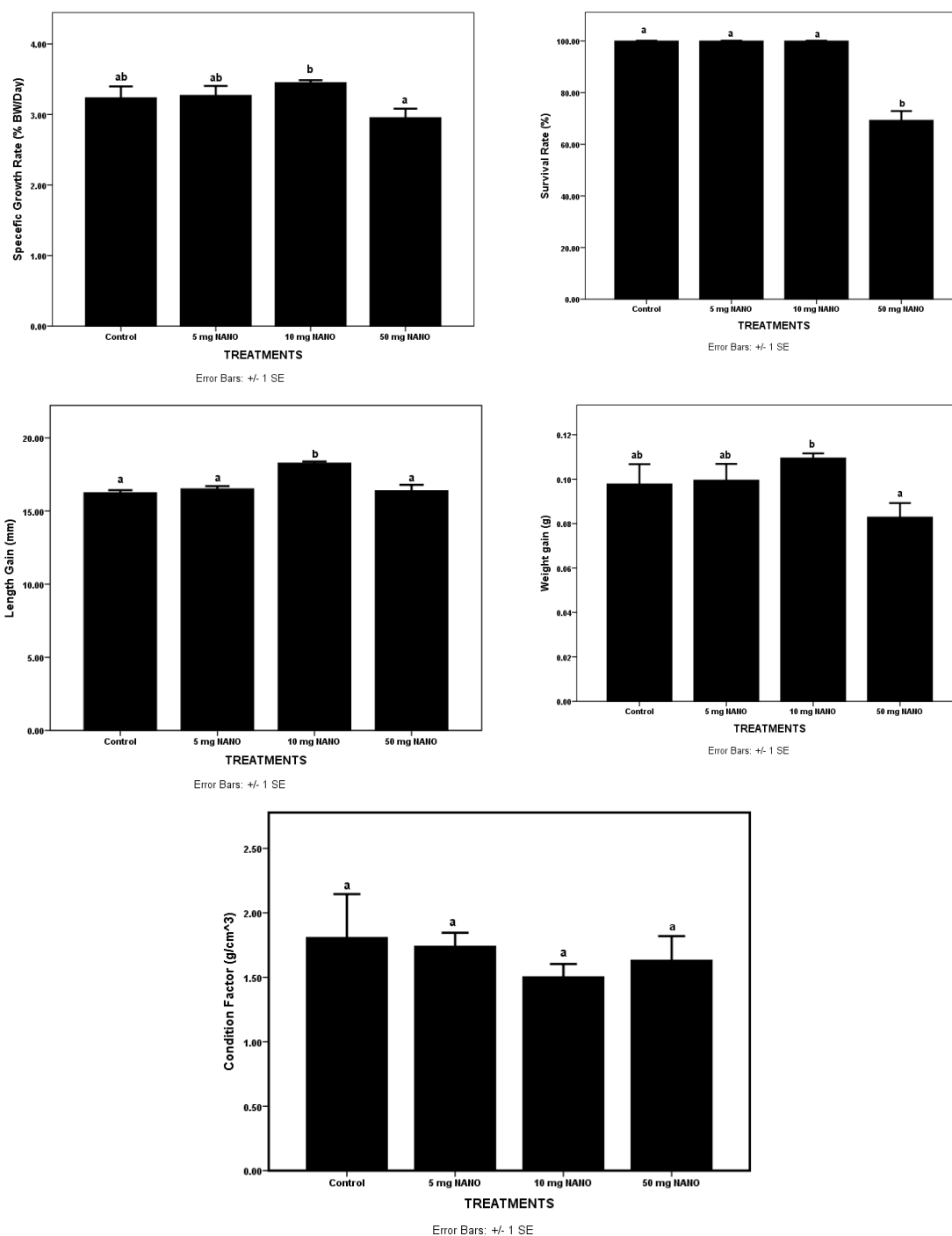
Figure 3: Growth factors and survival rate of guppy fed with different levels of selenium nanoparticles (Mean±S.E). Means with the same superscript are not significantly different (p>0.05).
