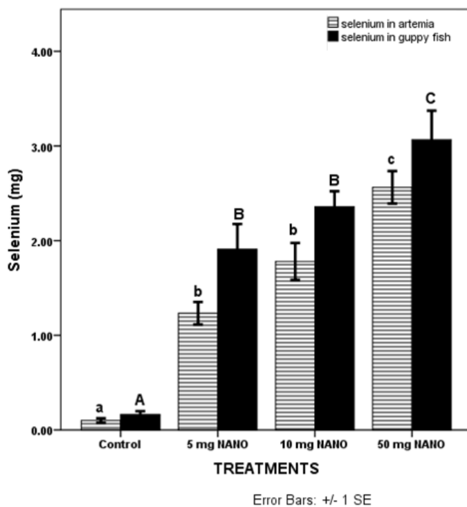
Figure 2: Selenium accumulation in Artemia nauplius and guppy larvae carcass at different treatments (Mean±S.E.). Means with the same superscript are not significantly different ( p>0.05 ).
