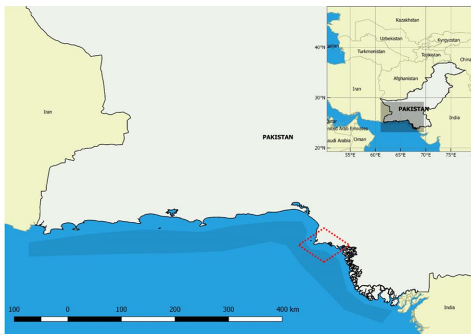
Figure 1: Red dotted area indicating main fish landing site (Karachi Fish Harbour) Paksitan
