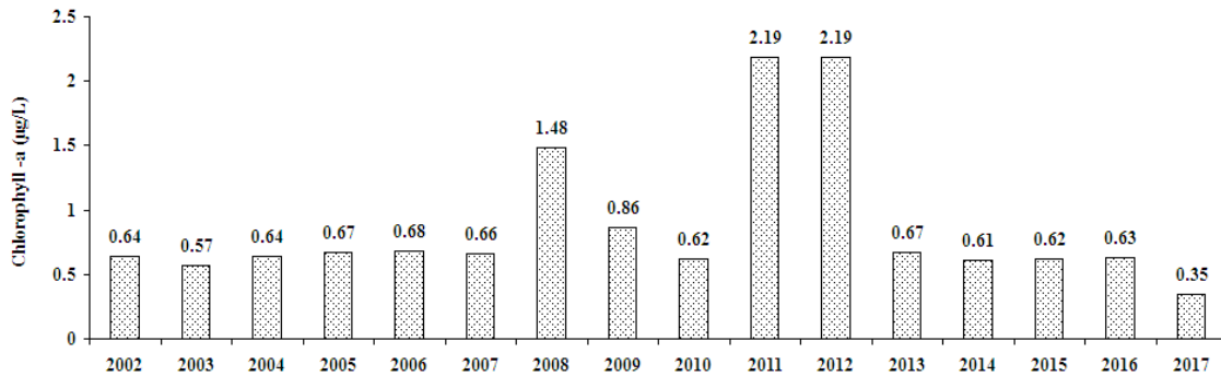
Figure 4: The average satellite-based Chlorophyll-a in the studied stations in Bushehr province waters, from 2002 to 2017.
