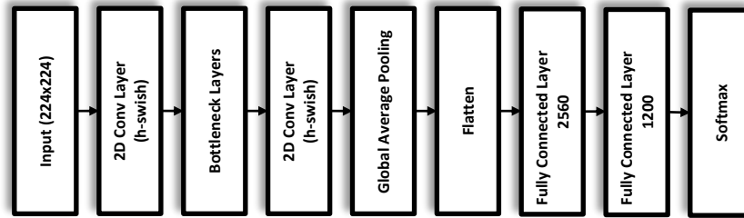
Figure 6: Schematic representation of our modified MobileNetV3-Small architecture.
